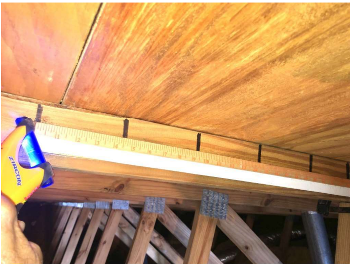
8d nails spaced 6" on center truss per code
